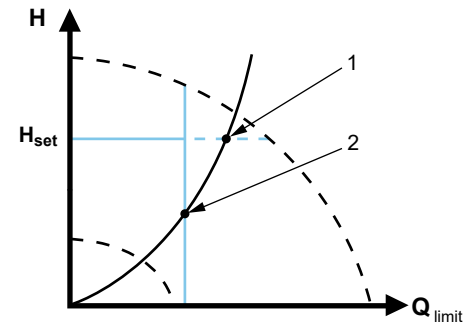
Constant-pressure control with FLOWLIMIT
