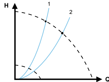
Hydraulic difference between the pump head to the right (1) and to the left (2) of the flap valve
