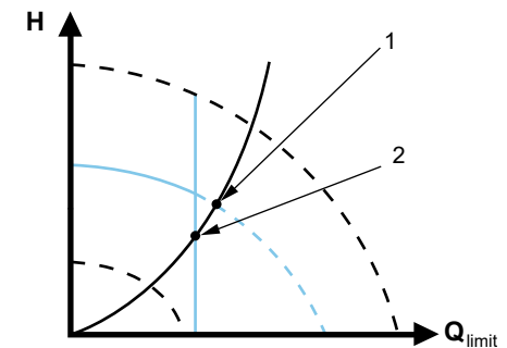
Constant curve with FLOWLIMIT
