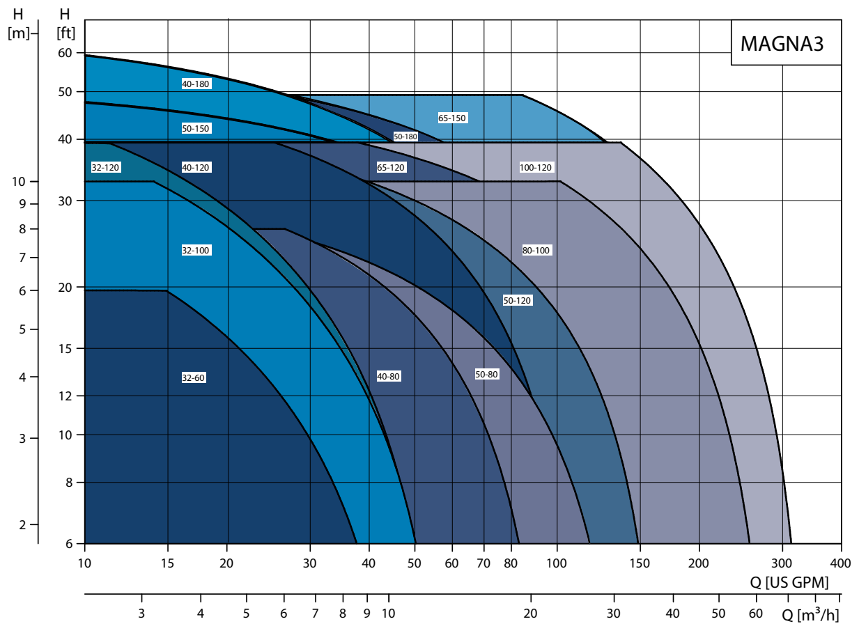
Performance range for MAGNA3 single-head pump
