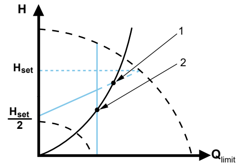
Proportional-pressure control with FLOWLIMIT
