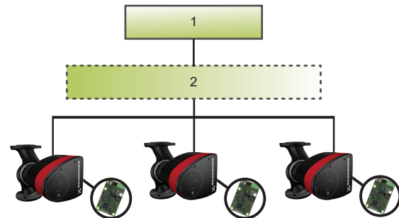
Example of typical building management system, BMS (1) with pumps connected in parallel. The gateway (2) facilitates the transfer of data between two different networks based on different communication protocols.
