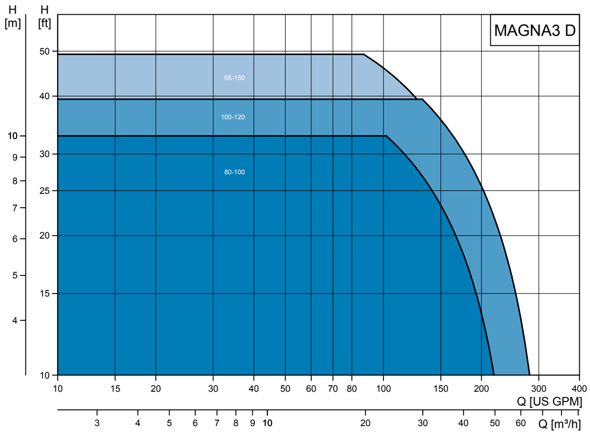
Performance range for MAGNA3 D twin-head pump in single-head operation
