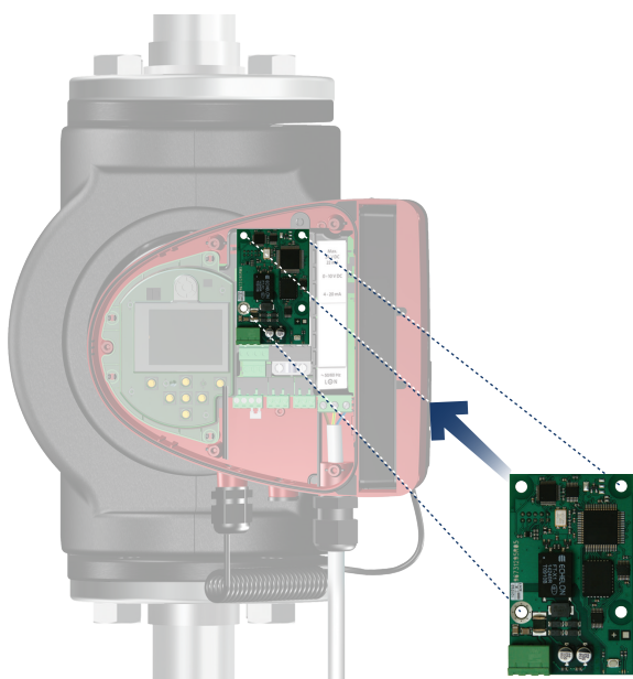
Location of the add-on CIM module in MAGNA3
