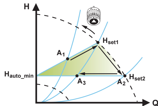
AUTOADAPT control
