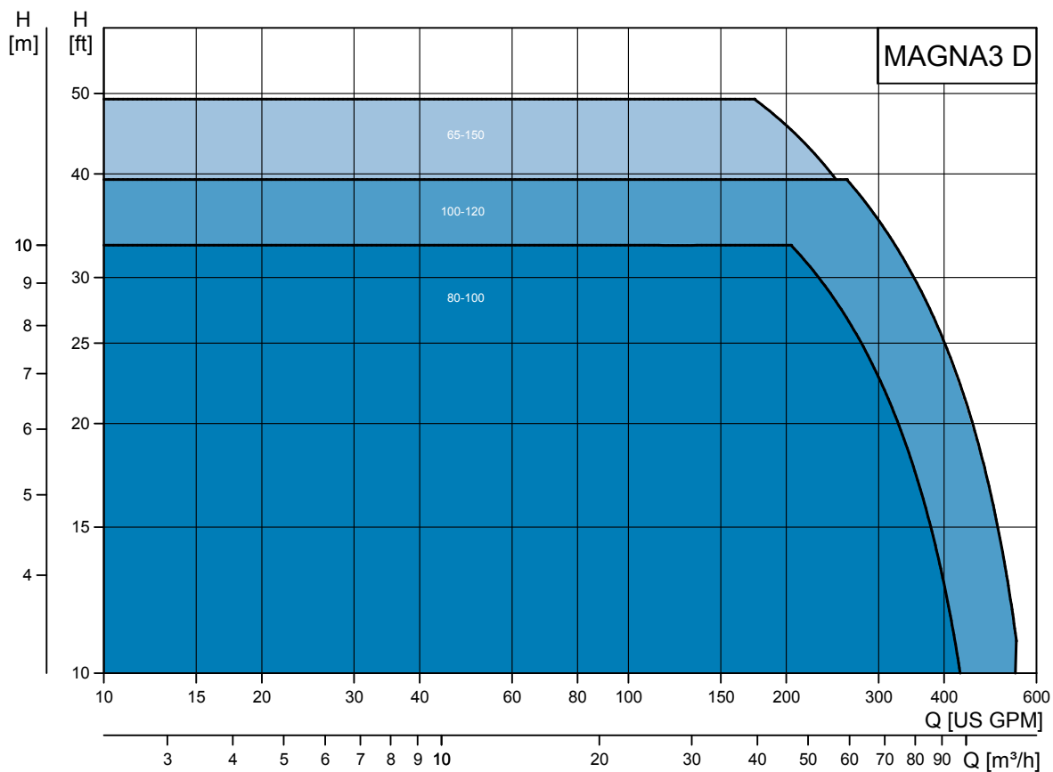
Performance range for MAGNA3 D twin-head pump in twin-head operation
