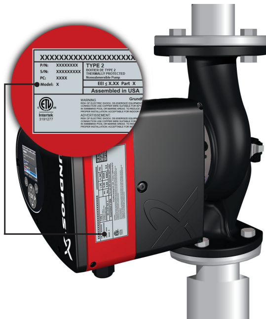
Location of the pump version on the nameplate
