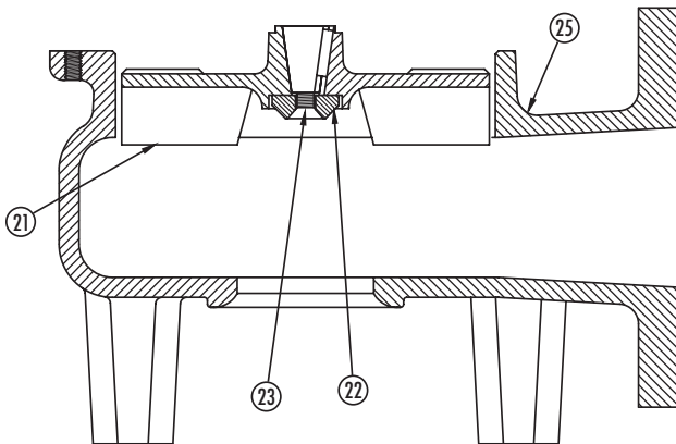
3RMW 1750 RPM
