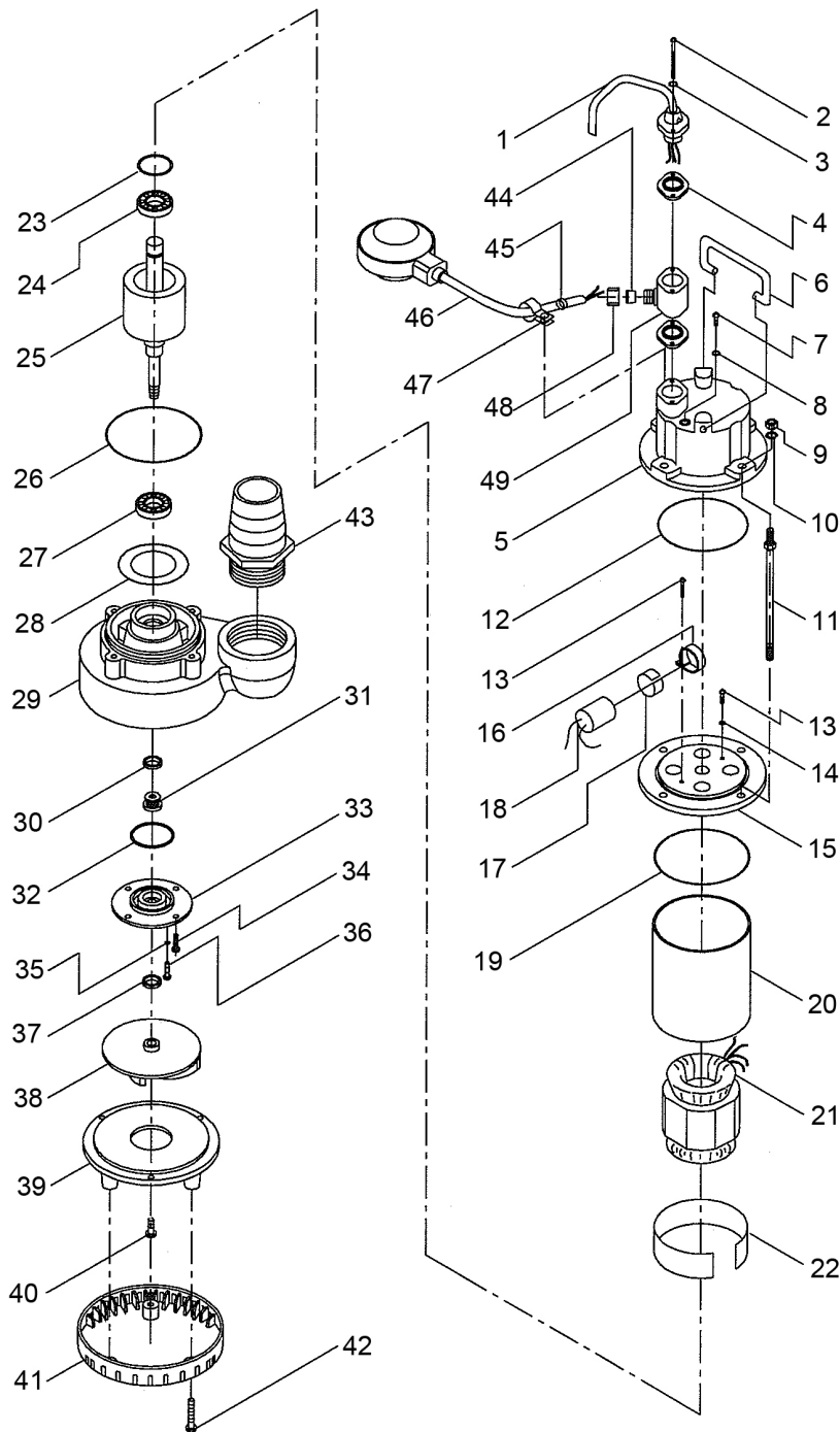
Figure 2 - Repair Parts Illustrations - 5980-95B & 598A-95B
