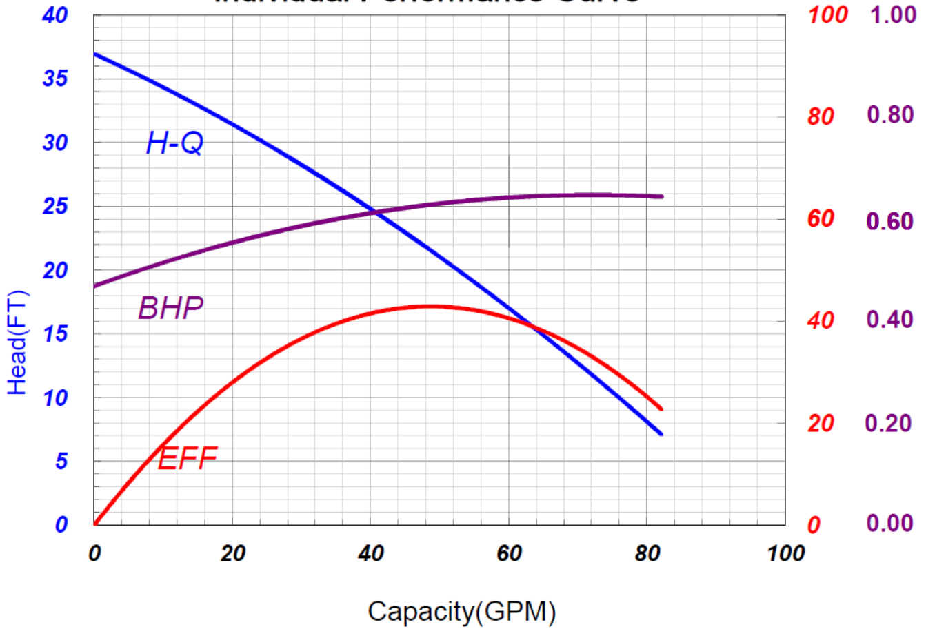
Stancor Model SC-50 Individual Performance Curve
