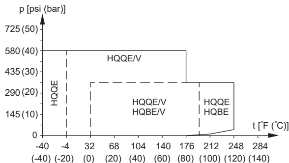
Operating range of standard shaft seals for Ø28 and Ø36 for CR 125-255, 100-300 HP (75-224 kW)
