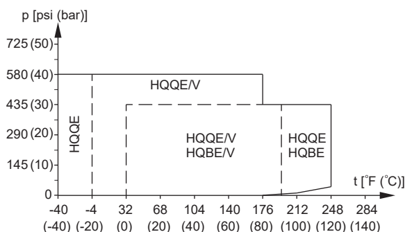
Operating range of standard shaft seals for CR, CRN 95-255, 15-75 HP (11-55 kW)
