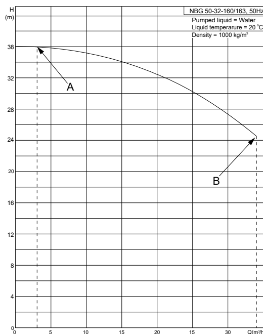
Example from Grundfos Product Center in www.grundfos.com showing minimum and maximum flow rate
