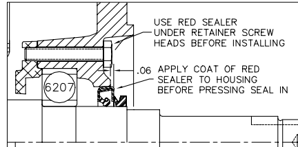
PULLEY END SEAL AND SLINGER DETAIL
