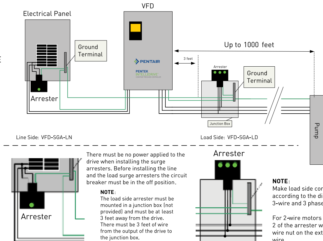
PENTEK INTELLIDRIVE Surge Arrester Connection Diagram
