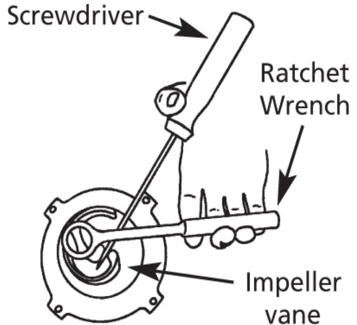
Figure 1 - Impeller Removal
