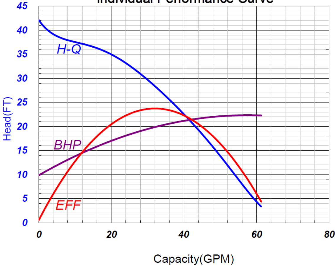
Stancor Model AHS-05 Individual Performance Curve
