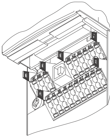
Fig. 38 Signal terminals
