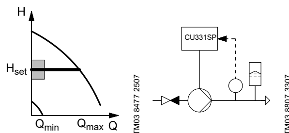
Fig. 24 Constant pressure with stop function
