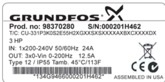
Fig. 21 Example of nameplate
