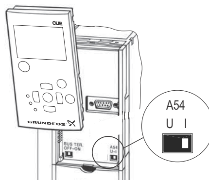
Fig. 36 Setting contact A54 to current signal "I"
