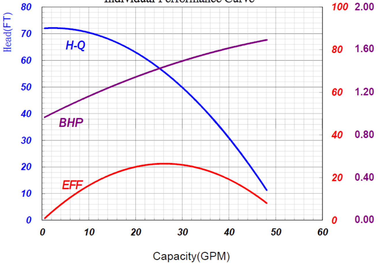
Stancor Model SG-150 Individual Performance Curve
