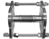
Fig. 58 Example of metal expansion joint
