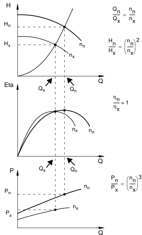
Fig. 49 Affinity equations
