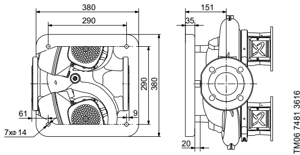
Drawing, TPE3 D 80
