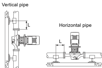
Fig. 51 Pump suspended directly in the pipes
