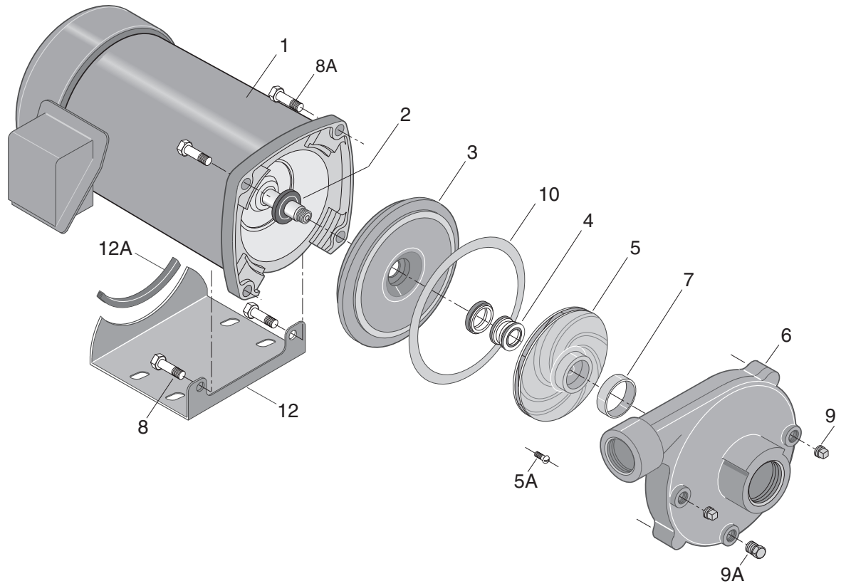
Capscrew Configuration
