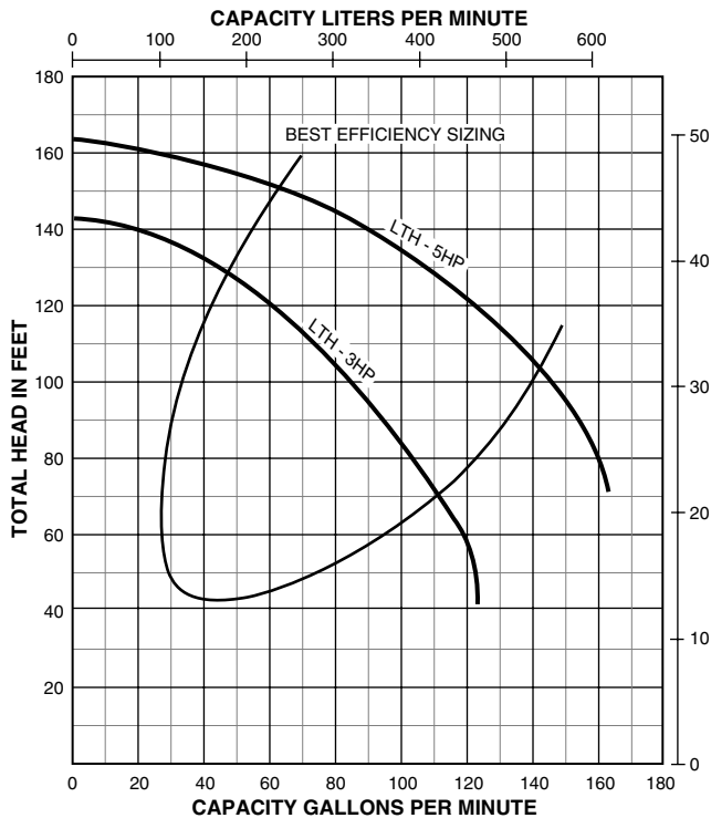
PUMP PERFORMANCE - LTH HIGH HEAD
