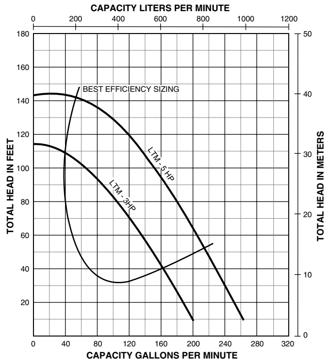
PUMP PERFORMANCE - LTM MEDIUM HEAD
