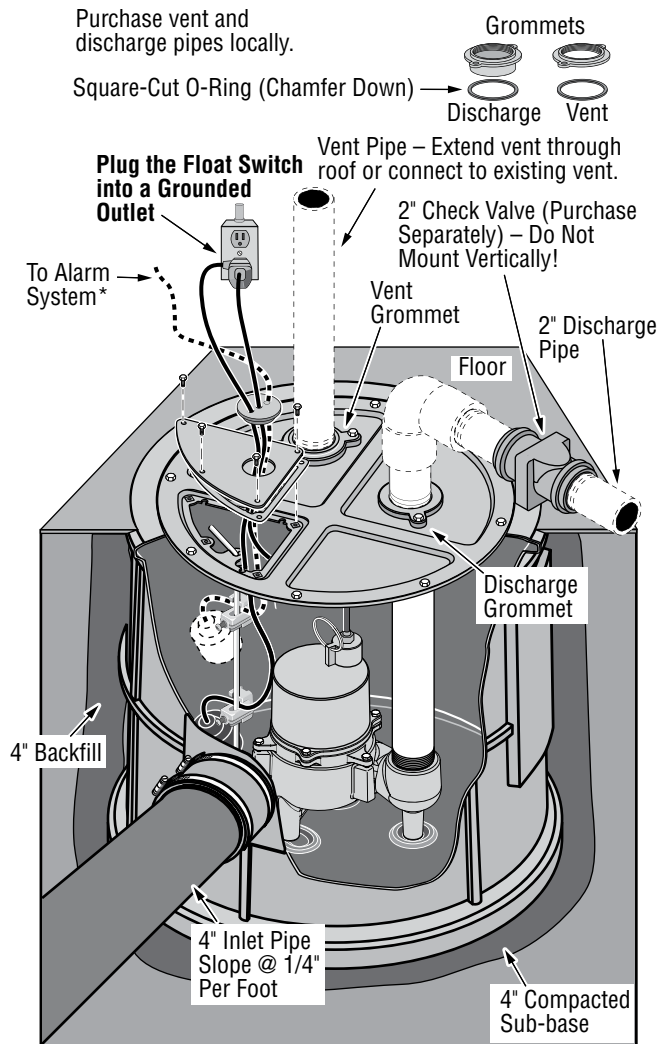
Figure 1 – Typical Installation
