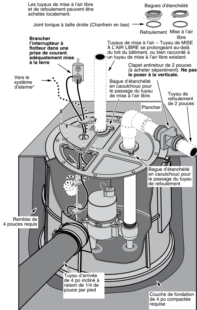
Figure 1 – Installation type
