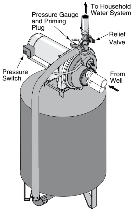
Figure 6: Pre-charged Tank Connections
