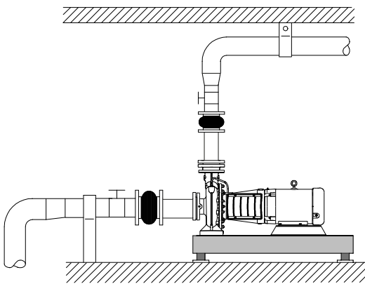
Pump installation
