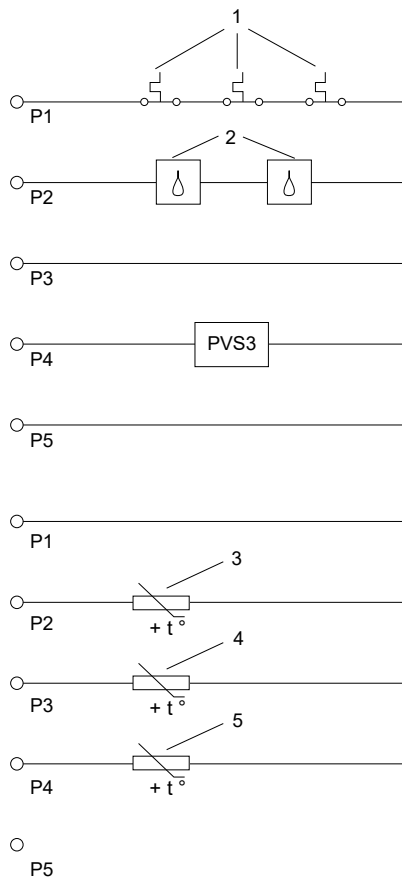
Sensor 2 and Sensor 2 Ex, double cable
