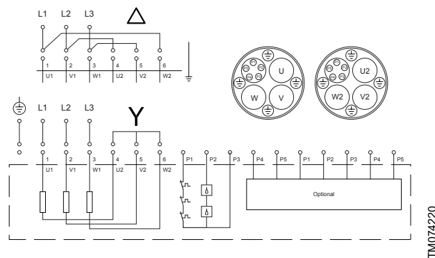
18-wire / EMC double cable
