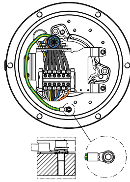
Earthing screw, standard
