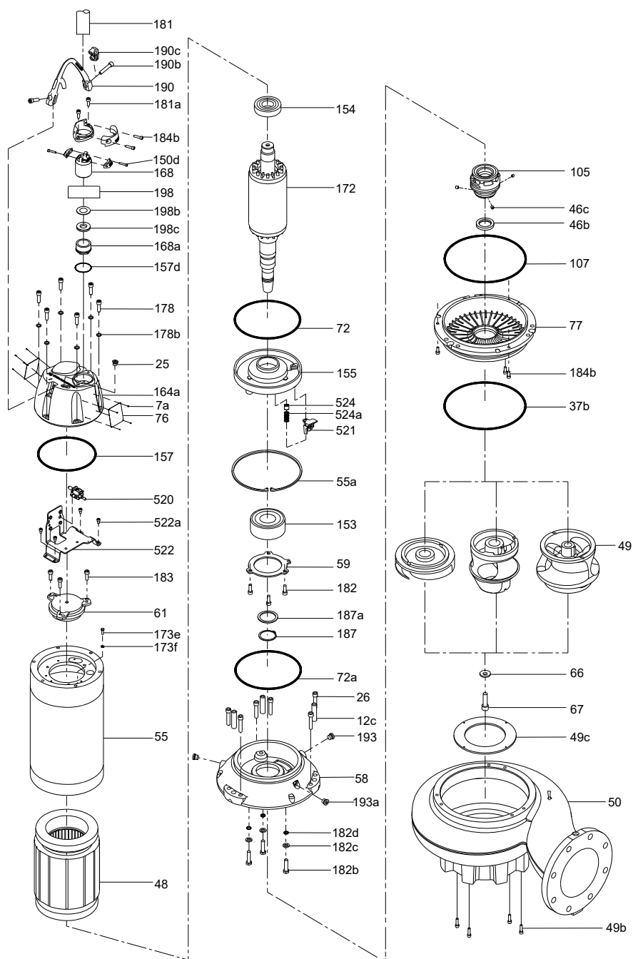
SLV, SL, SL1, SL2 pumps, 2-4 poles
