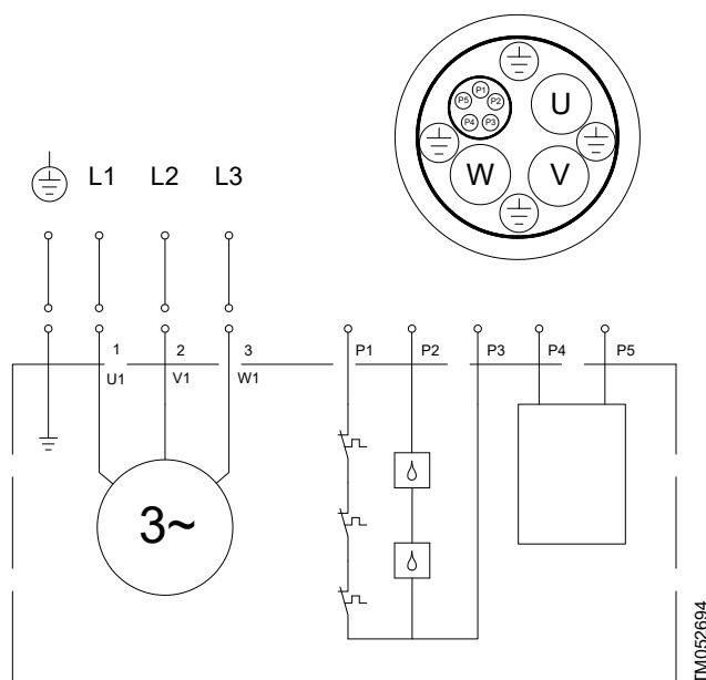
8-wire, EMC cable
