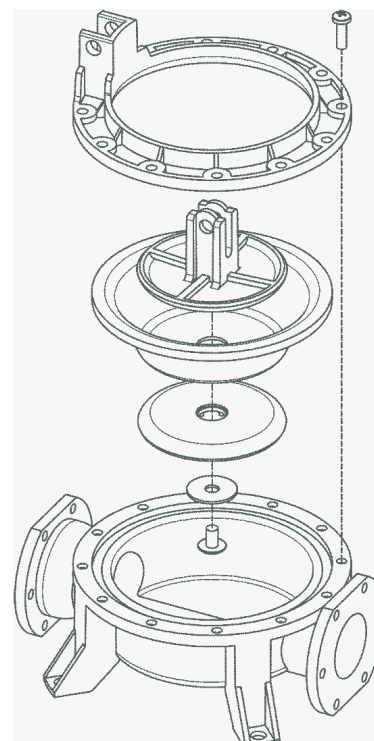
Figure 1 – Diaphragm Assembly
