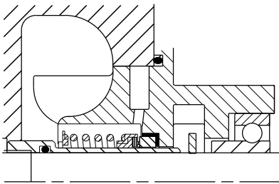
Fig. 17 Rubber bellows shaft seal
